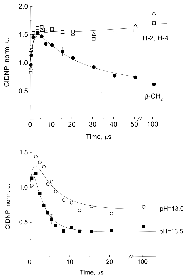
Figure 4. (a) 1 H CIDNP kinetics obtained during the irradiation of a solution containing 5.8 \times 10^{-4} M 2,2'-dipyridyl and 0.14 M N -acetyl histidine (pH = 5.3): \Delta , H-2; \square , H-4; \bullet , \beta -CH 2 of N -acetyl histidine. Solid lines: calculations as described in the text using the parameters R_0 = 1.2 \times 10^{-4} M, T_1 = 16 \mu s (H-2, H-4), T_1 = 196 \mu s ( \beta -CH 2 ), k_t = 2.0 \times 10^9 M -1 s -1 . (b) 1 H CIDNP kinetics for H-2 of N -acetyl histidine, obtained during the irradiation of a solution containing 1.4 \times 10^{-2} M 2,2'-dipyridyl and 1.6 \times 10^{-2} M N -acetyl histidine: \circ , pH = 13.0; \blacksquare , pH = 13.5. Solid lines: calculations as described in the text using the parameters R_0 = 2.2 \times 10^{-4} M (pH = 13.0), R_0 = 3.5 \times 10^{-4} M (pH = 13.5), T_1 = 16 \mu s, k_t = 2.0 \times 10^9 M -1 s -1 , k_{ex} = 1.5 \times 10^8 M -1 s -1 .
